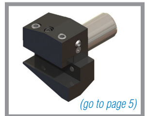
Part #: VDI30-ID20MZ-OHC4 Left Hand Inverted Axial Turning Tool
