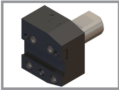
Part #: VDI40-CO32MX-LH
