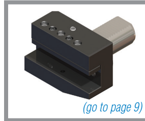
Part #: VDI40-OD10X-LG-OHB8 Left Hand Long Inverted Radial Turning Tool
