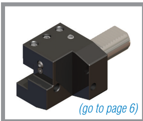
Part #: VDI30-BG12Z-C-E2 Double External Coolant Flow Boring Bar Holder
