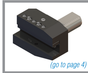
Part #: VDI30-OD75X-LG-B6 Left Hand Long Radial Turning Tool
